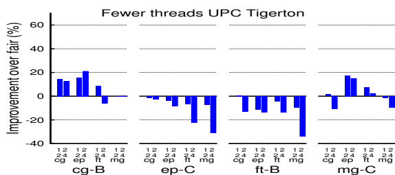
Figure 18. Relative differences in performance when the application is given fewer threads. x-axis presents the number of application and co-runner threads. (1/2 and 2/4).
