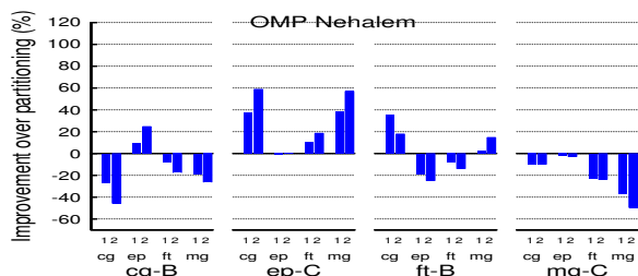
Figure 13. Performance for OMP benchmarks when sharing the system compared to partitioning.
