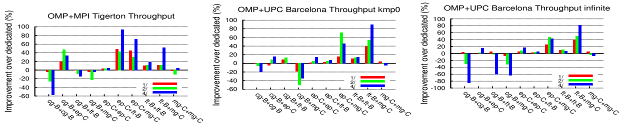
Figure 16. Throughput for OMP/UPC sharing. KMP\_BLOCKTIME=0 .
