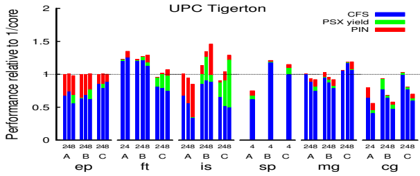
Figure 3. UMA oversubscription UPC. Performance is normalized to that of experiments with 1 task per core. Number of tasks per core can be 2, 4 or 8. SP requires a square number of threads. Overall workload performance varies from -2% to 2%.
