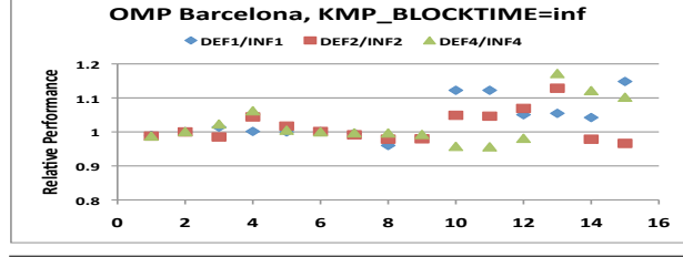
Figure 10. OpenMP performance with “non-cooperative” synchronization on Barcelona. DEF1/INF1 stands for the default/kmp=inf value with one thread per core. Values greater than 1 indicate performance improvement.
