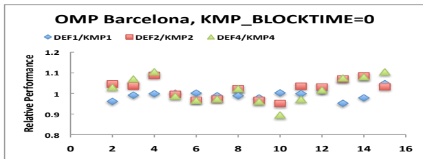
Figure 9. OpenMP performance with cooperative synchronization on Barcelona. DEF1/KMP1 stands for the default/kmp=0 value with one thread per core. Values greater than 1 indicate performance improvement.
