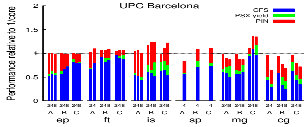
Figure 4. NUMA oversubscription UPC. Performance is normalized to that of experiments with 1 task per core. Number of tasks per core can be 2, 4 or 8. SP requires a square number of threads. Overall workload performance varies from -2% to 2%.
