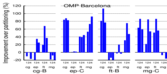
Figure 11. Performance for OMP benchmarks when sharing the system compared to partitioning.
