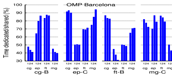
Figure 12. Percentage of performance sharing compared with dedicated one per core. The benchmarks are sharing the whole system.
