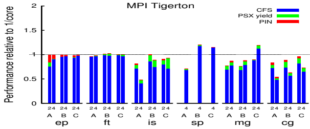
Figure 7. UMA oversubscription MPI. Performance is normalized to that of experiments with 1 task per core. Number of tasks per core can be 2 or 4. Overall workload performance decreases by 10% to 18%.
