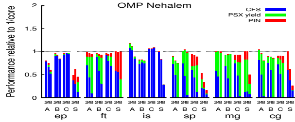
Figure 8. NUMA oversubscription OpenMP. Performance is normalized to that of experiments with 1 task per core. Number of tasks per core can be 2, 4 or 8. Workload performance decreases by 6% to 14%.
