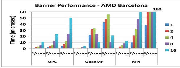
Figure 1. Barrier performance with oversubscription at different core counts (legend) on AMD Barcelona. Similar results are observed on all systems.
